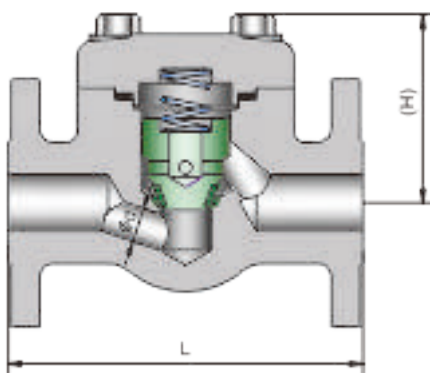
PISTON TYPE CHECK VALVE
